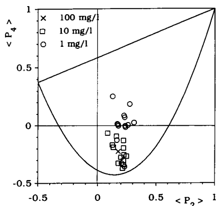
FIGURE 5 Order parameters for \text{H}_2\text{TMPyP} adsorbed on glass from solutions of various porphyrin concentrations. The physical boundaries of \langle P_2 \rangle and \langle P_4 \rangle are indicated by solid lines.
