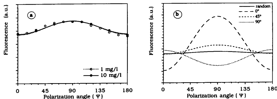
FIGURE 4 Fluorescence signal of \text{H}_2\text{TMPyP} adsorbed on glass as a function of the polarization angle \Psi of the incident light beam. (a) Experimental points for adsorption from solutions of 1- and 10-mg/l \text{H}_2\text{TMPyP} in 10-mM phosphate buffer pH 7. The curves through the points are obtained by fitting with F(\Psi) = A + B \cos^2(\Psi) . (b) Calculated curves for a random distribution and sharp distributions with orientation angle \theta = 0^\circ , 45^\circ , and 90^\circ .
