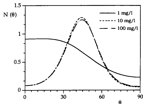
FIGURE 6 Orientation distribution functions of \text{H}_2\text{TMPyP} adsorbed on glass, corresponding to the average values for \langle P_2 \rangle and \langle P_4 \rangle for adsorption from solutions with porphyrin concentrations of 1, 10, and 100 mg/l and calculated following the maximum-entropy method.
