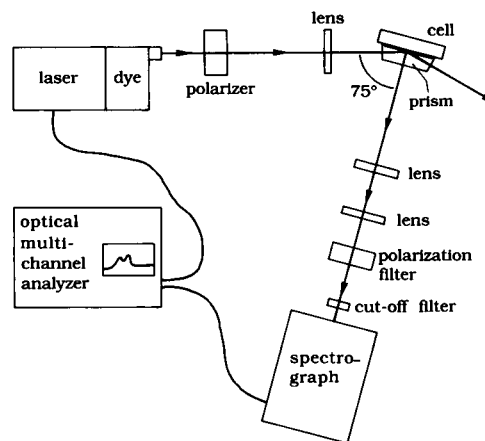
FIGURE 3 Schematic diagram of the TIRF setup.
